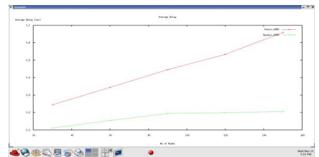
Figure 1.7: Average delay for static and dynamic AODV
