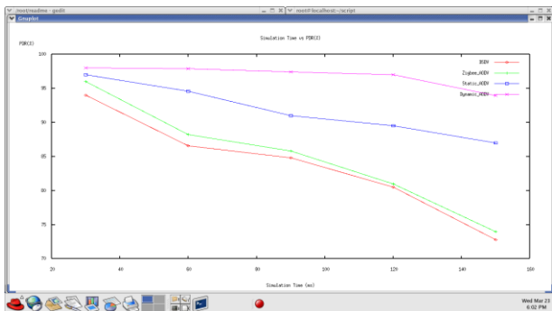
Figure 1.10: Packet delivery ratio VS simulation time
